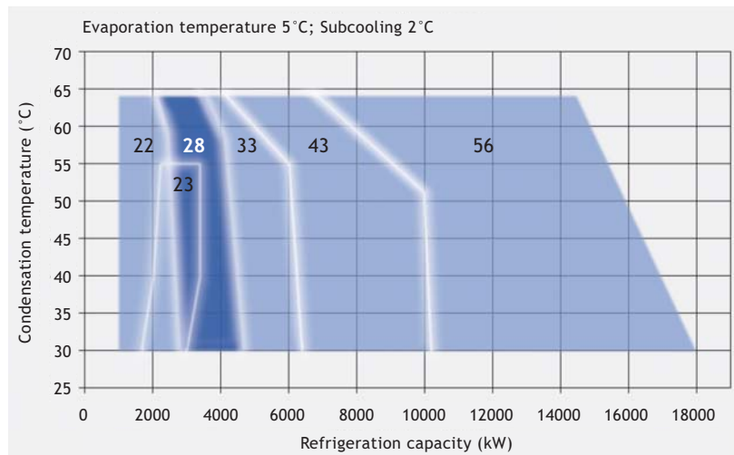
Uniturbo® range of compressors, marked in dark blue the data for Uniturbo® 28
